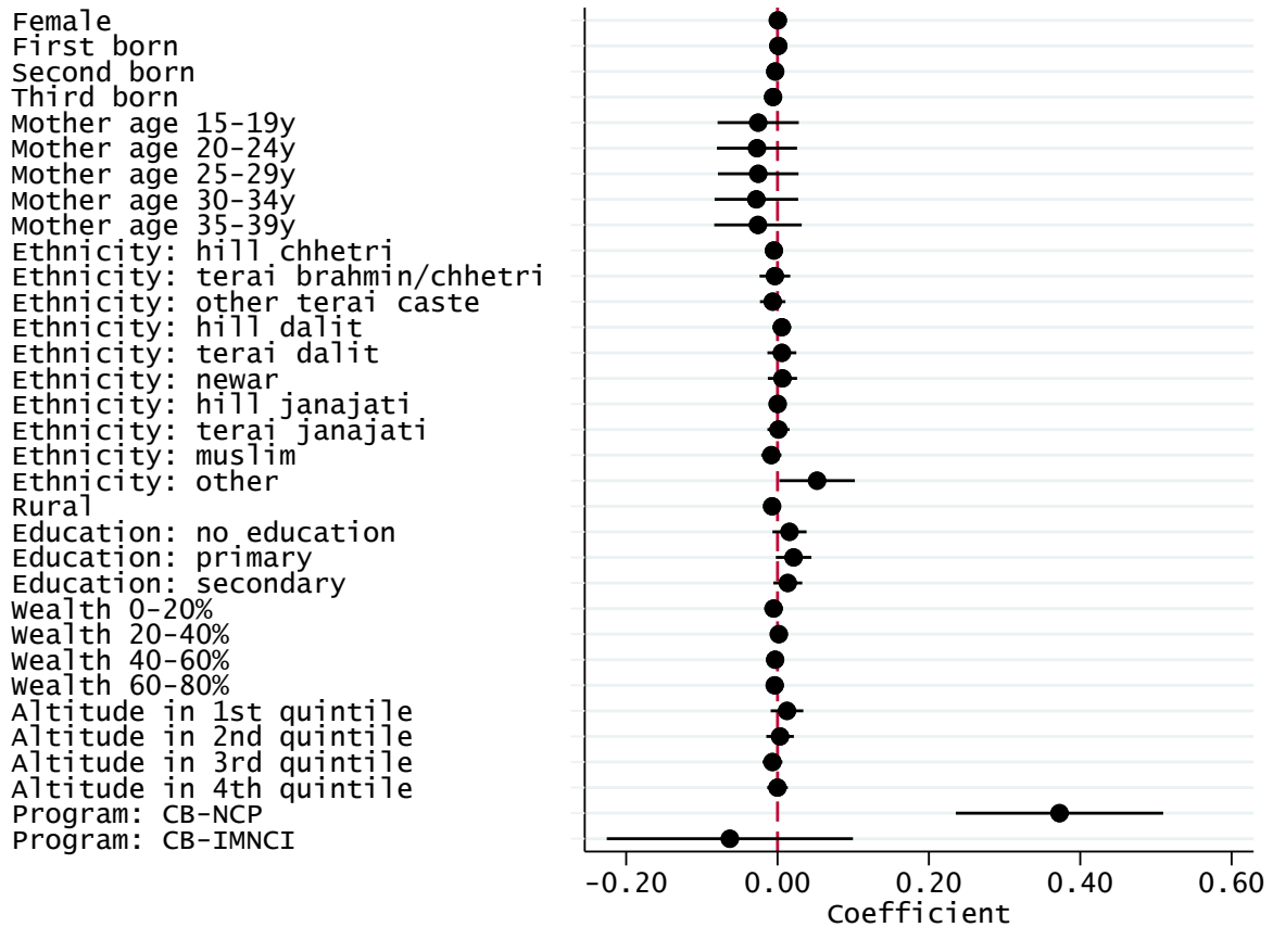
Figure 2: Covariate balance
